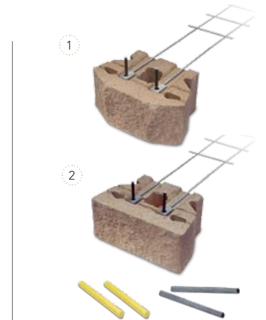
2 Connection/Steel pins required per unit.
